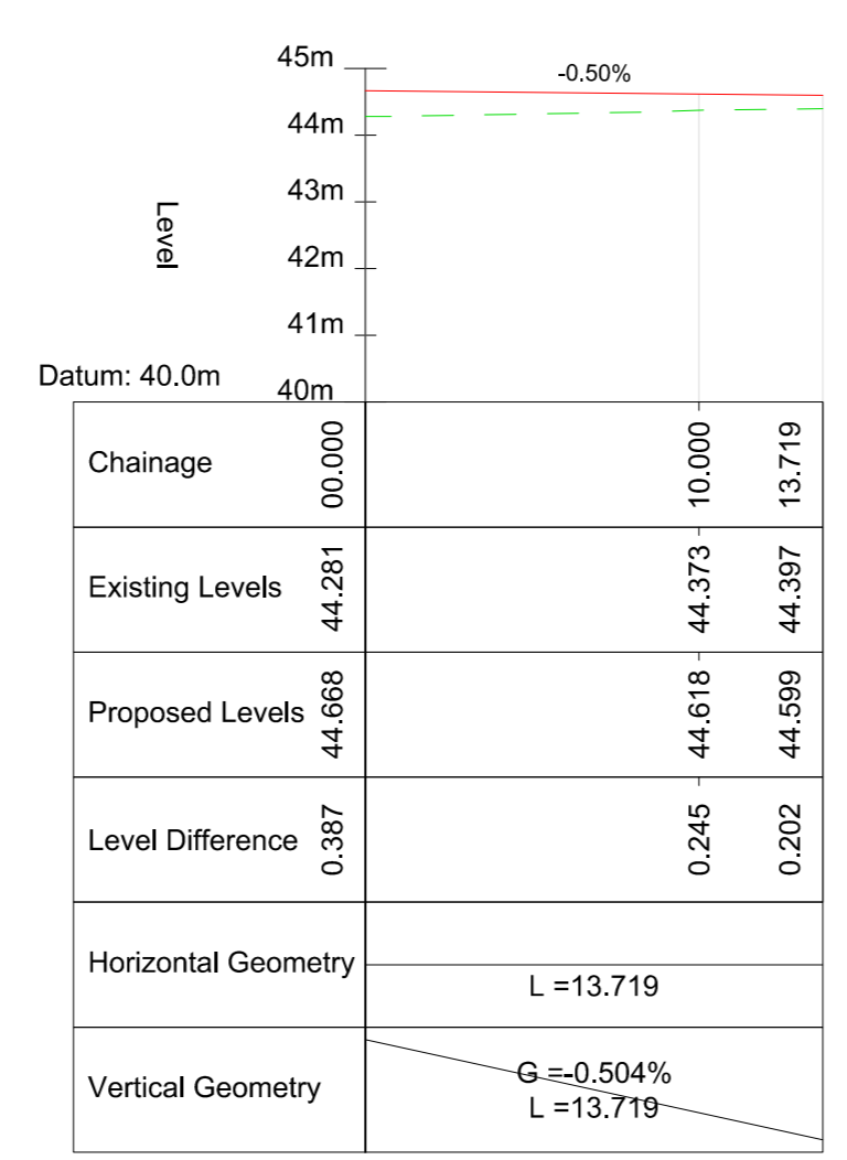
BM-Road 5-1 SCALE @ A0: H=1:250; V=1:125 SCALE @ A2: H=1:500; V=1:250
