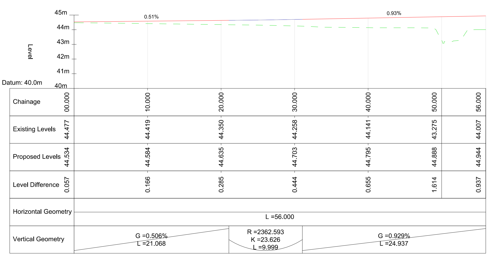
BM-Road 5 SCALE @ A0: H=1:250; V=1:125 SCALE @ A2: H=1:500; V=1:250
