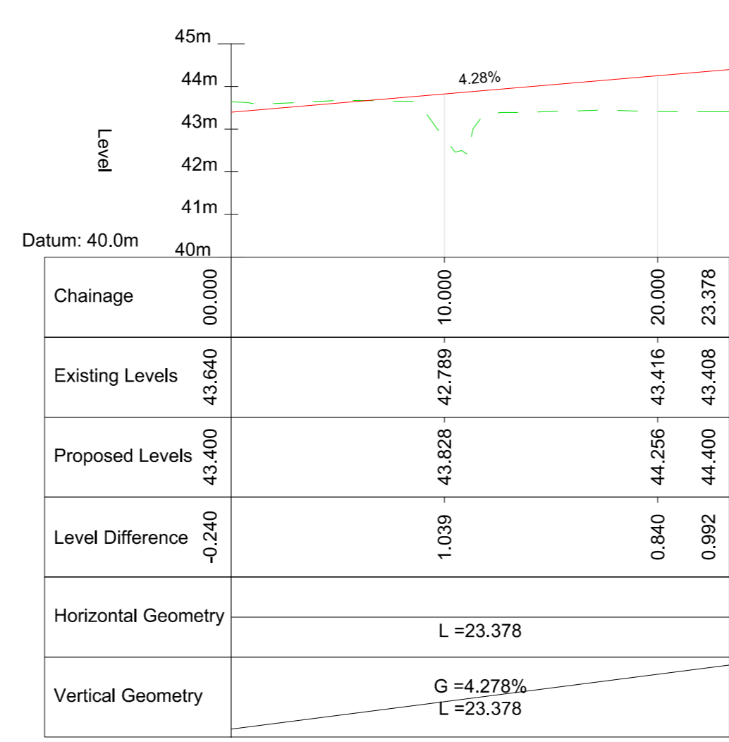
BM-Road 6 SCALE @ A0: H=1:250; V=1:125 SCALE @ A2: H=1:500; V=1:250
